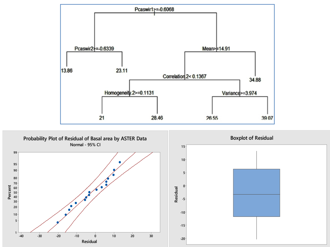
Supplementary Figure S3. Binary regression tree (top) and probability (left), and box plot (right) of residual CART model for basal area/ha using ASTER data.
