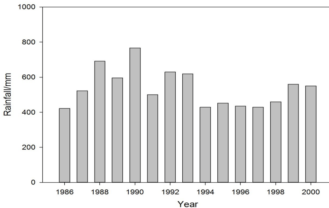
Supplementary Figure S1. Average annual precipitation in the Luoyugou watershed.
