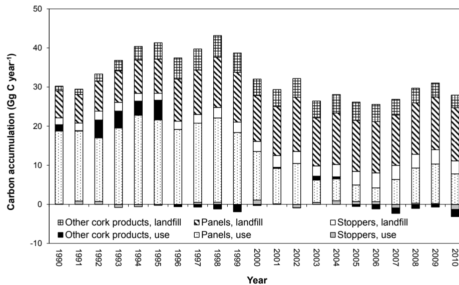
Supplementary Figure S2. Contribution of each pool of cork products to carbon accumulation estimated with the SCA.
