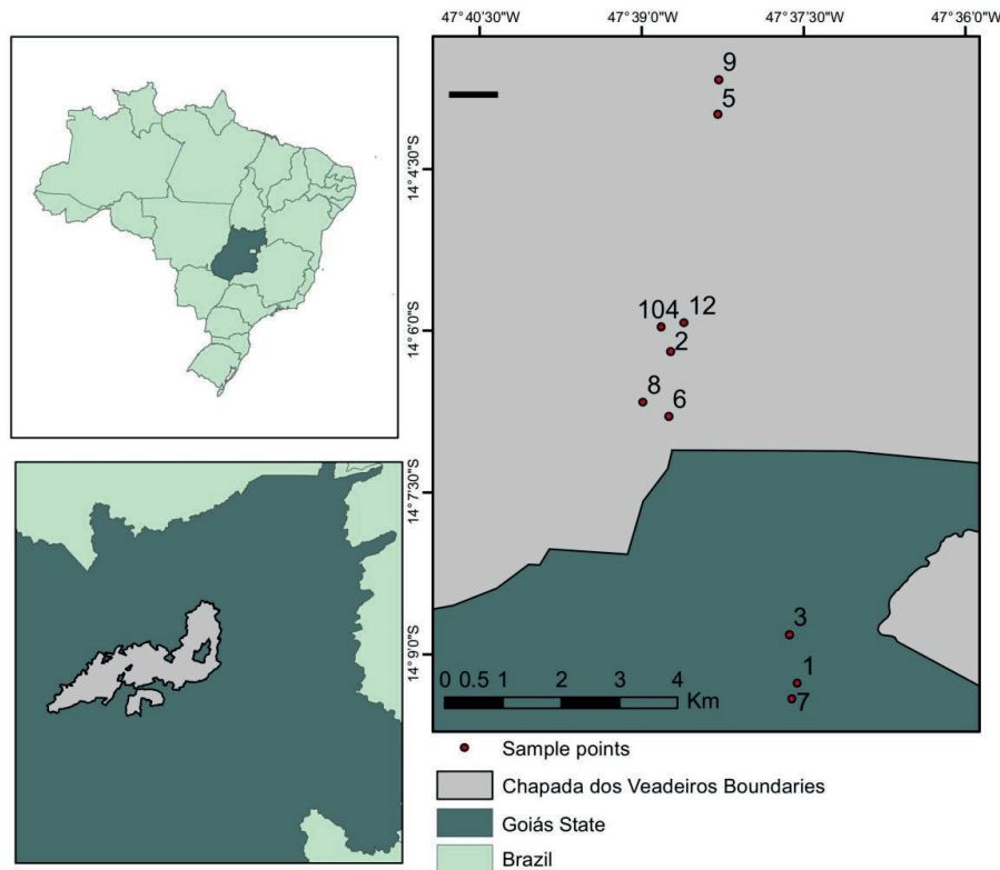
Figure 1. Chapada dos Veadeiros National Park, in Goiás State, Brazil, including phytophysiognomies with and without burning: 1, Campo Limpo without burning; 104, Campo Limpo with burning; 3, Campo Sujo without burning; 12, Campo Sujo with burning; 5, Cerrado sensu stricto without burning; 6, Cerrado sensu stricto with burning; 7, Cerradão without burning; 8, Cerradão with burning; 9, Veredas without burning; 2, Veredas with burning.
