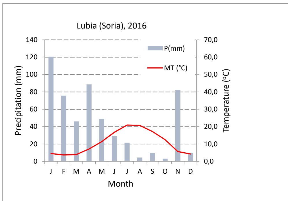
Figure S1: Atmospheric characterisation during 2016 in study area 1 (Lubia).
