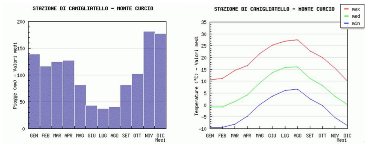
Figure S1. Precipitation (left) and temperature diagrams (minimum, average and maximum) (right) (survey station of Camigliatello Silano, province of Cosenza). (Font: Arpacal http://cfd.calabria.it , 2016).
