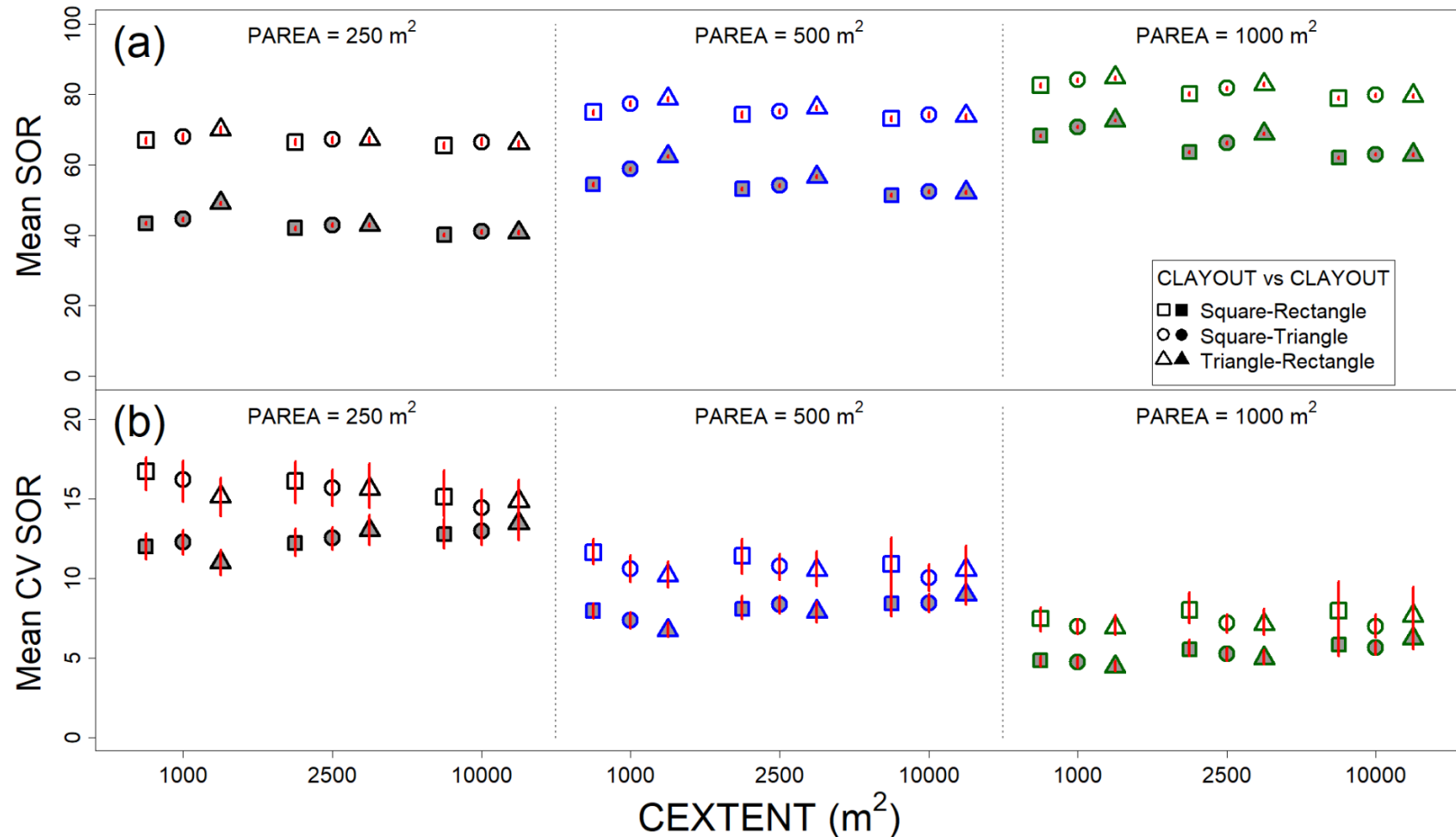
Figure S3. (a) Mean ( \bar{\theta} ) and (b) mean CV ( \overline{CV_{\theta}} ) Sørensen similarity index for comparing species composition between two cluster plots of two different cluster layouts for Fushan (open symbols) and Pasoh (filled grey symbols). The three comparisons are: (1) CLAYOUT = square vs CLAYOUT = rectangle ( \square and \blacksquare ), (2) CLAYOUT = square vs CLAYOUT = triangle ( \circ and \bullet ), (3) CLAYOUT = triangle vs CLAYOUT = rectangle ( \triangle and \blacktriangle ). The comparisons are controlled for PAREA and CEXTENT. PAREA are 250 (black symbols), 500 (blue symbols), and 1000 \text{m}^2 (green symbols). CEXTENT are 1000, 2500, and 10000 \text{m}^2 . Red solid lines depict empirical 95% confidence intervals.
