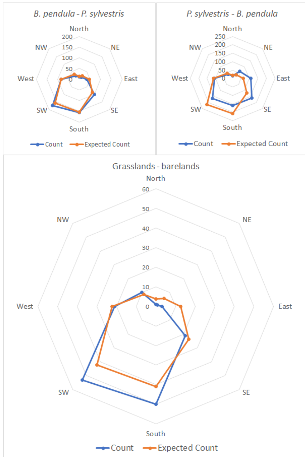
Figure S4. Graphs showing the distribution of points of two main species mixed forests and grasslands-barelands in relation to the expected values of chi-test for time period 1945-2009.
