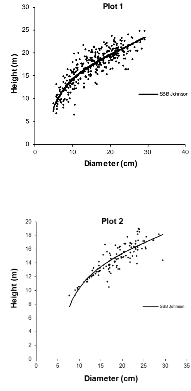
Figure S3. Scatter plot showing the line of the S_{BB} distribution from plot 1 and 2 in P. radiata using the indirect method fitted by CML.
